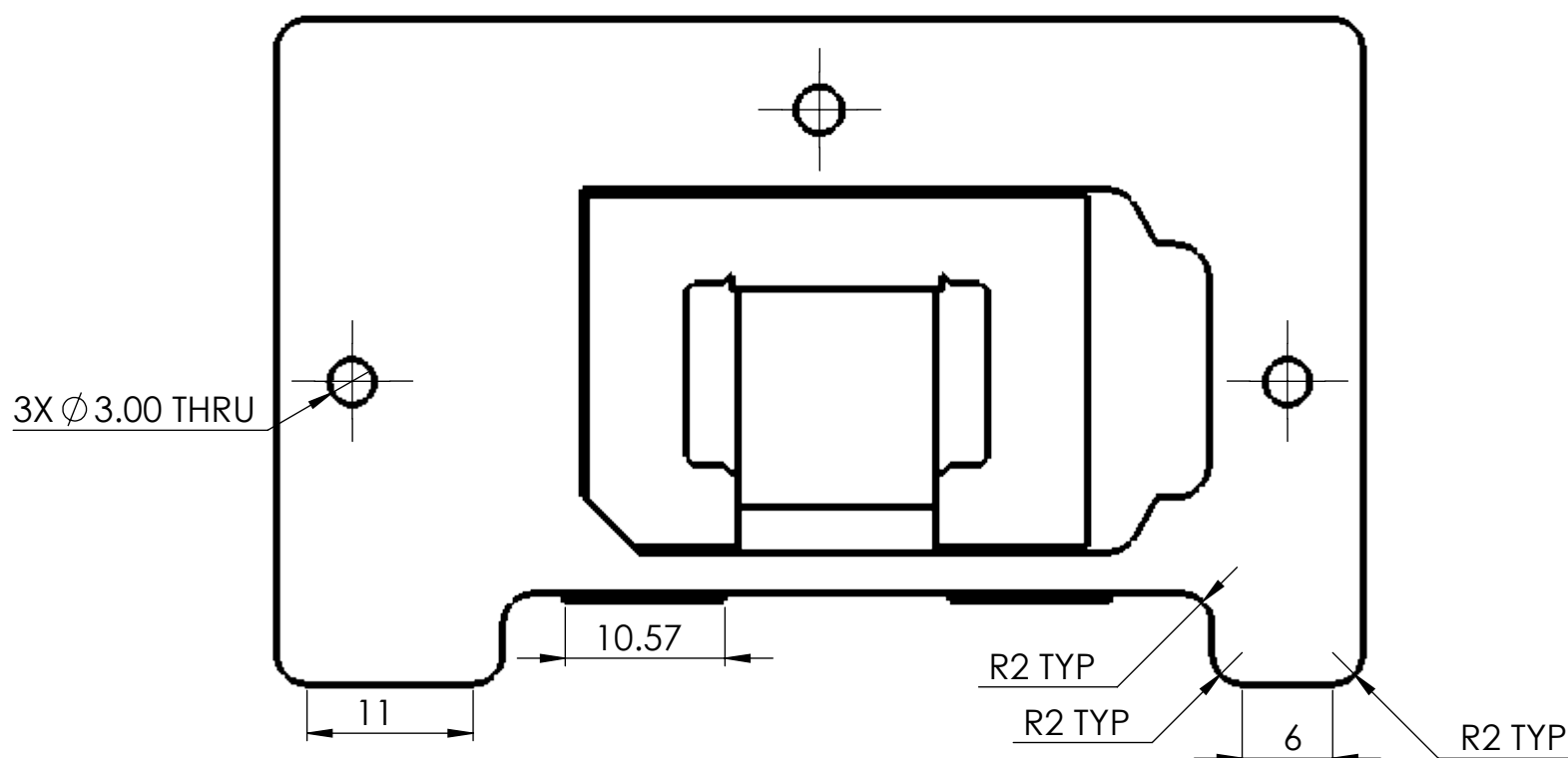
BACK VIEW
