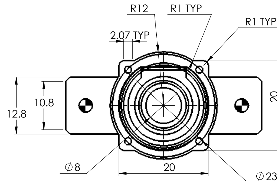
FRONT VIEW
