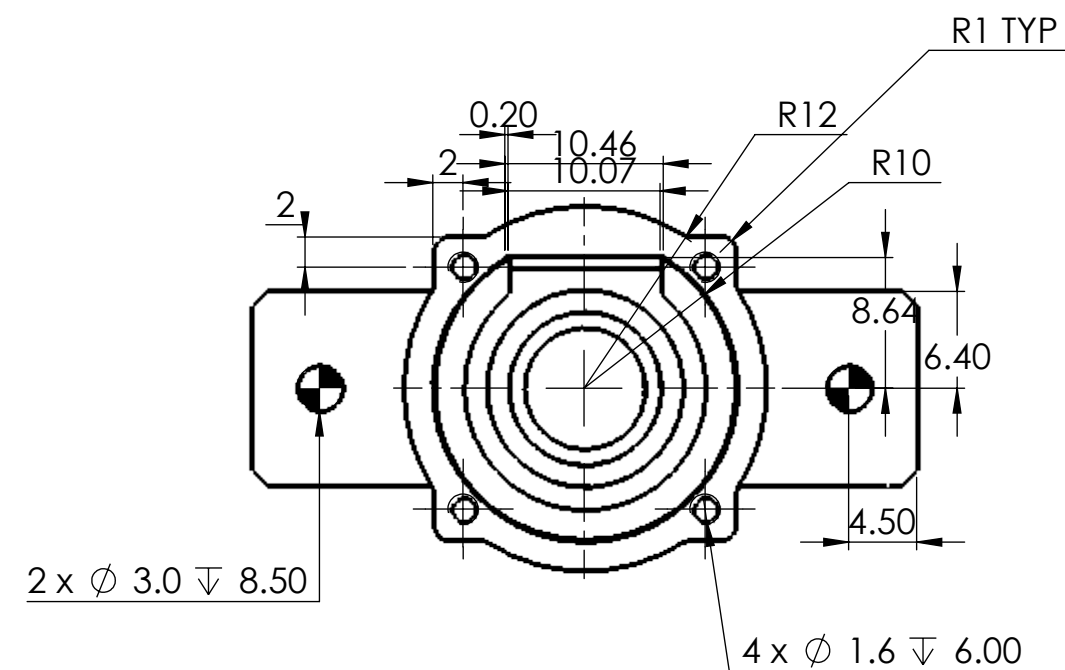
BACK VIEW
