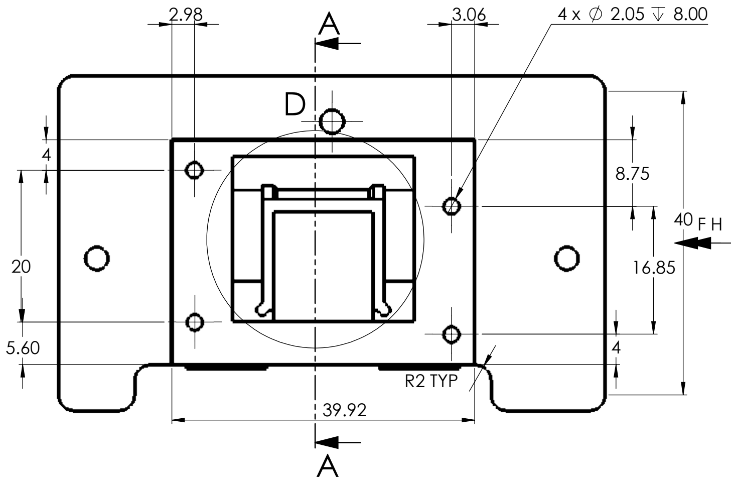
FRONT VIEW
