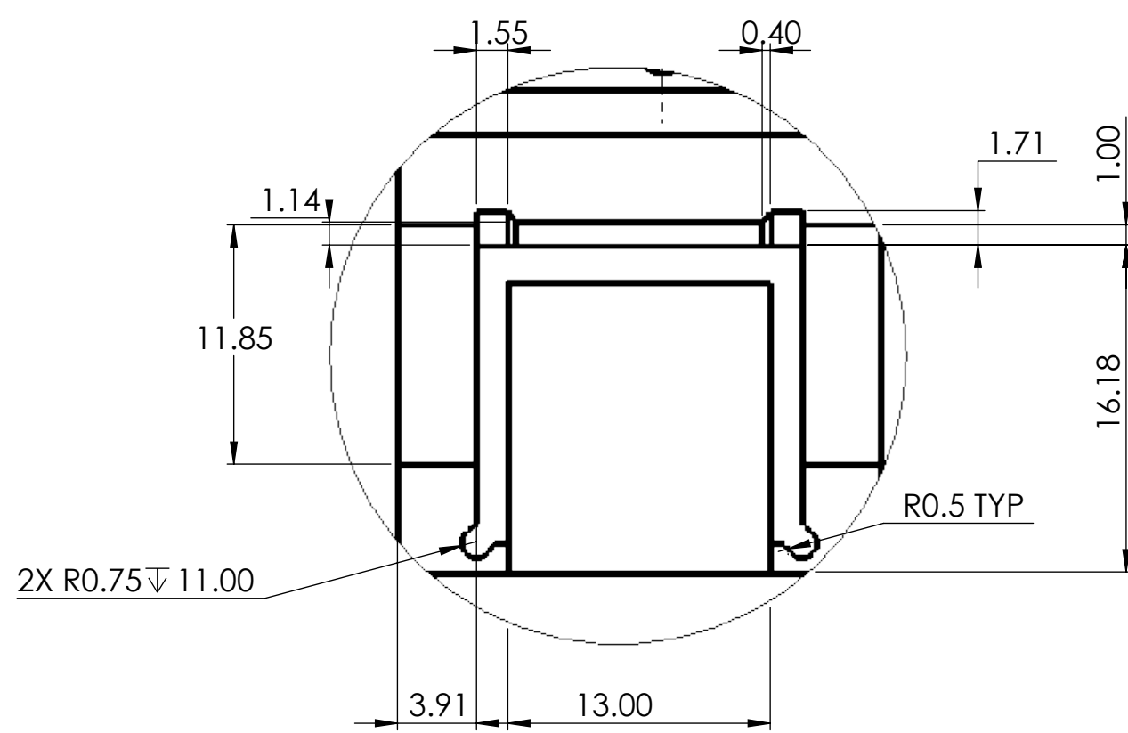
DETAIL D SCALE 3 : 1
