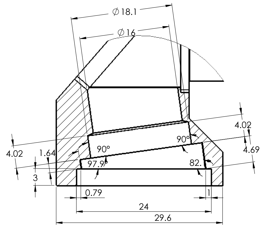
DETAIL X
