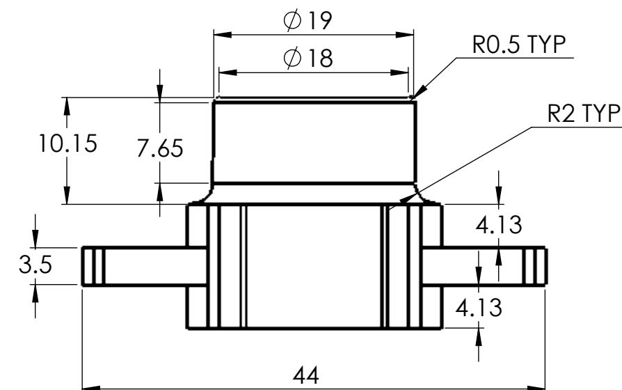
BOTTOM VIEW
