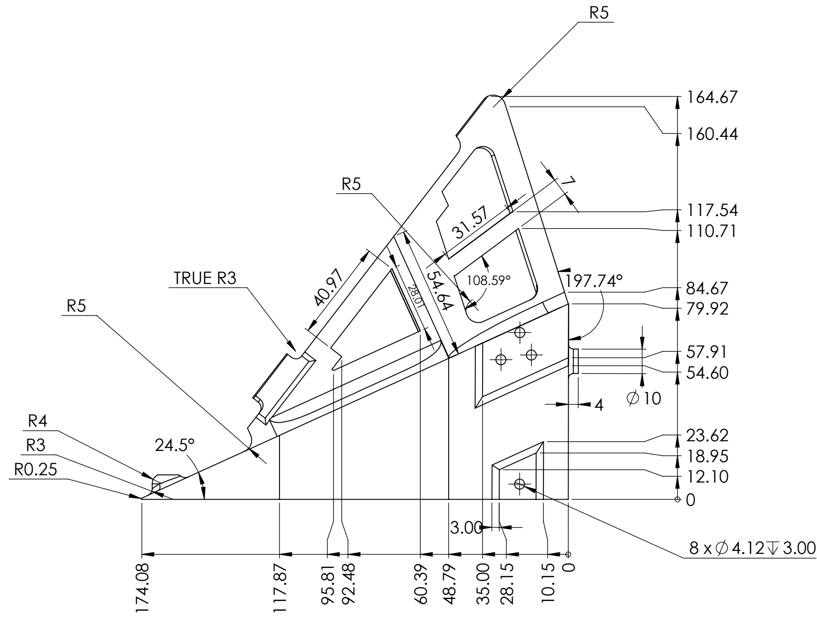
FRONT VIEW
