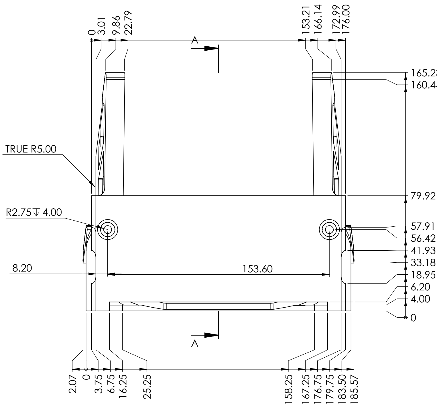
SIDE VIEW
