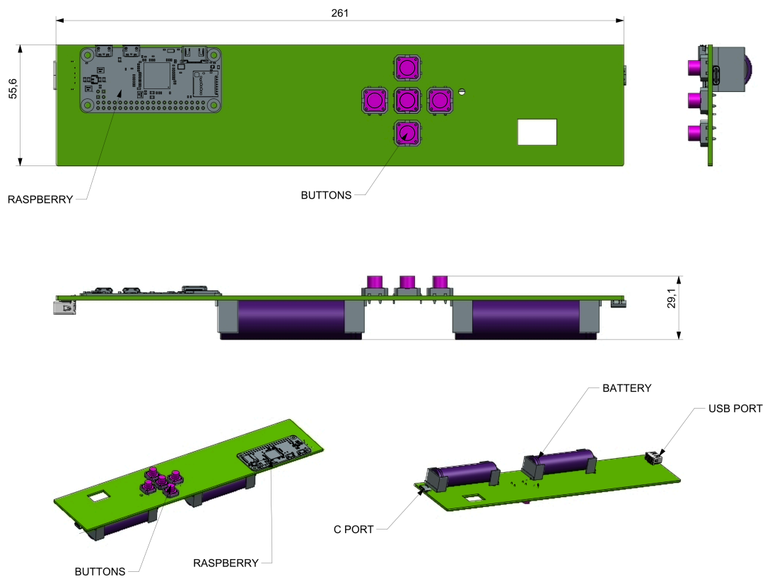
Figure 1: PCB Layout
