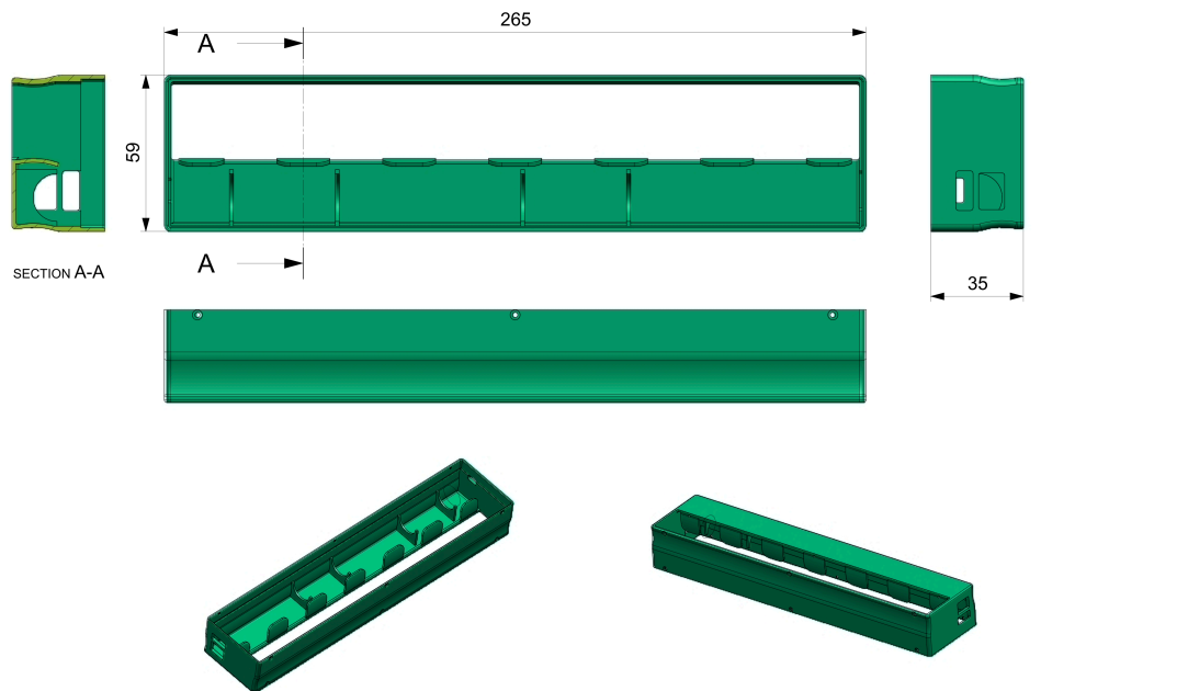
Figure 2: Chassis bottom part
