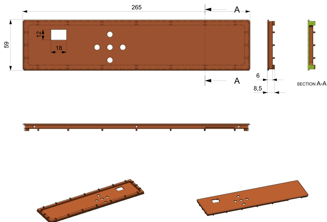
Figure 3: Chassis Top Part
