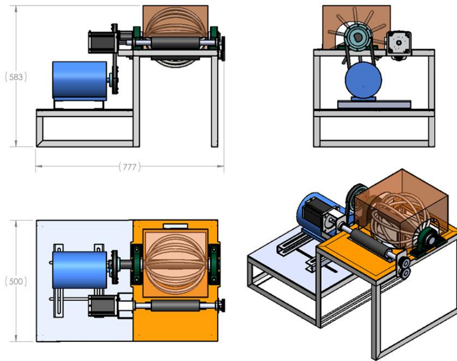
Trolley mountable decorticator unit
