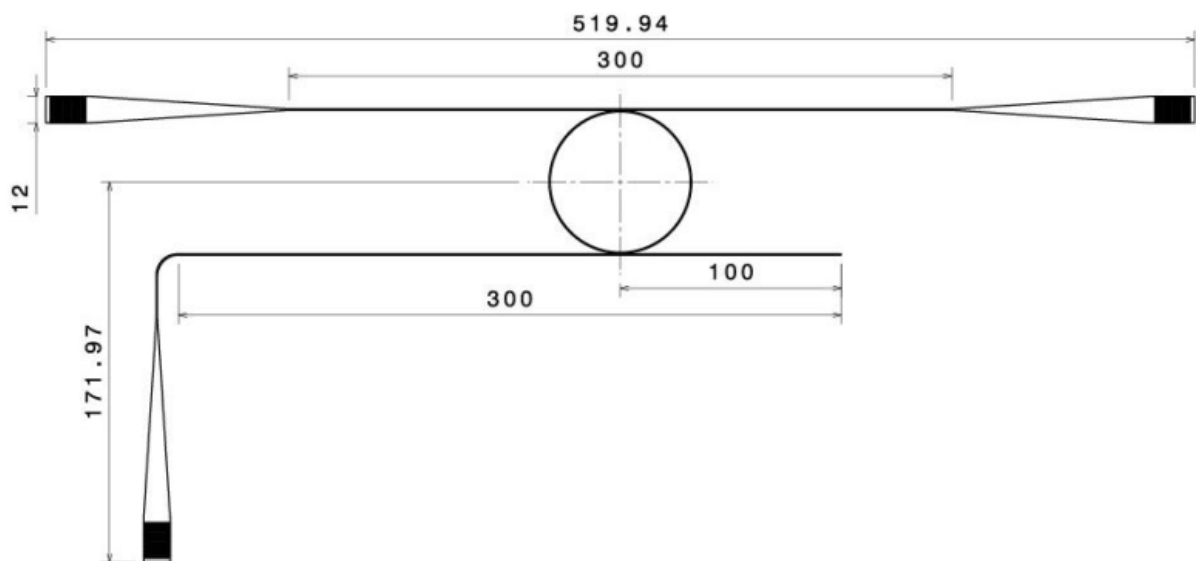
PIC Circuit (All units are in microns)
