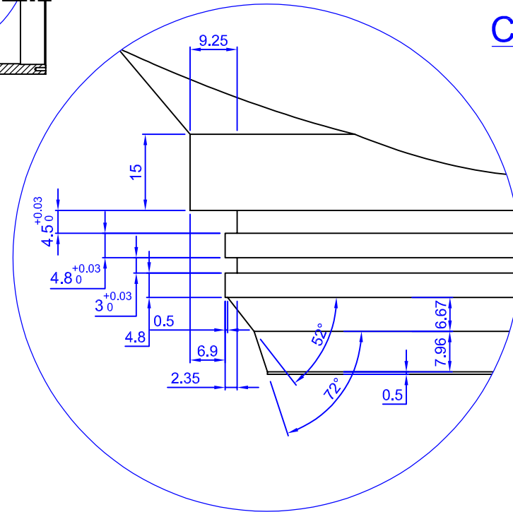
DETAIL C SCALE 6:1
