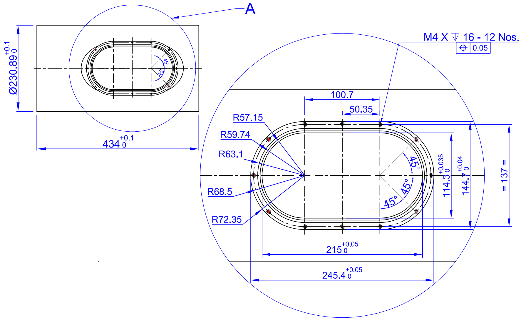
DETAIL A SCALE 2:1
