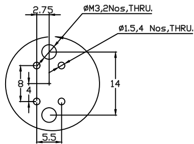
DETAIL OF B
