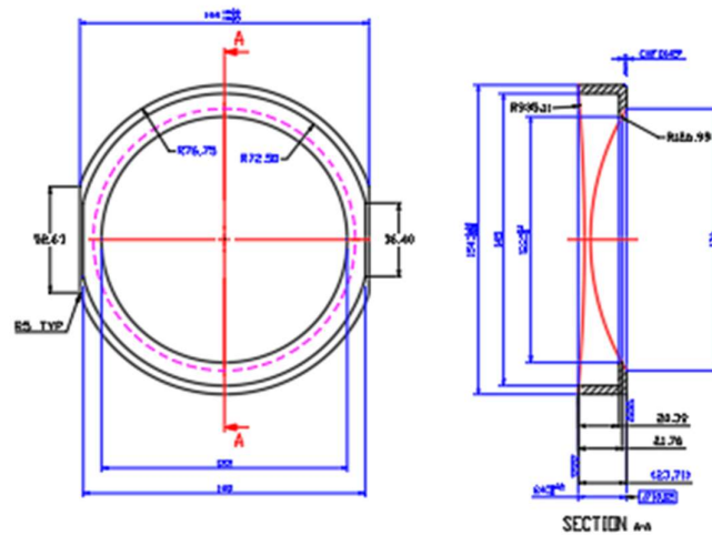
Figure 4: SPACER 1 @ 2NOS
