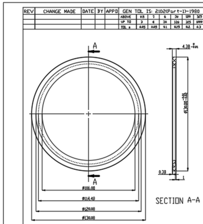
Figure 1: SPACER 2 @ 2NOS
